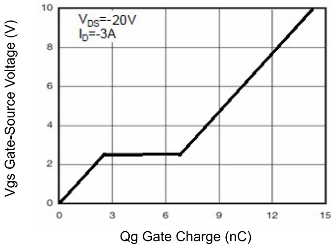
Figure 9 Gate Charge
