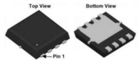
PDFN3.3X3.3-8L
