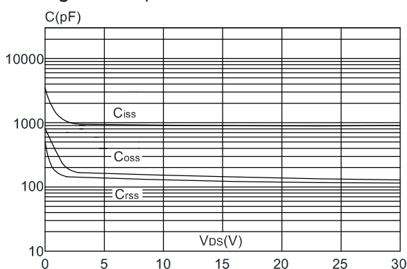
Figure 6: Capacitance Characteristics
