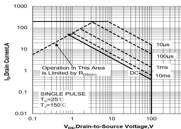
Figure 12. Maximum Safe Operating Area
