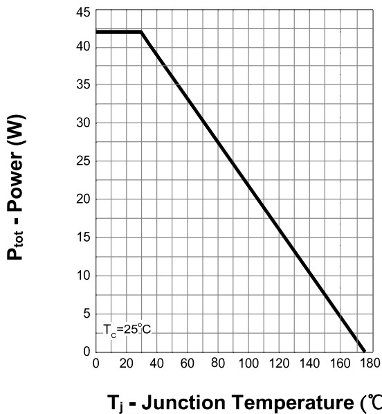
Power Dissipation
