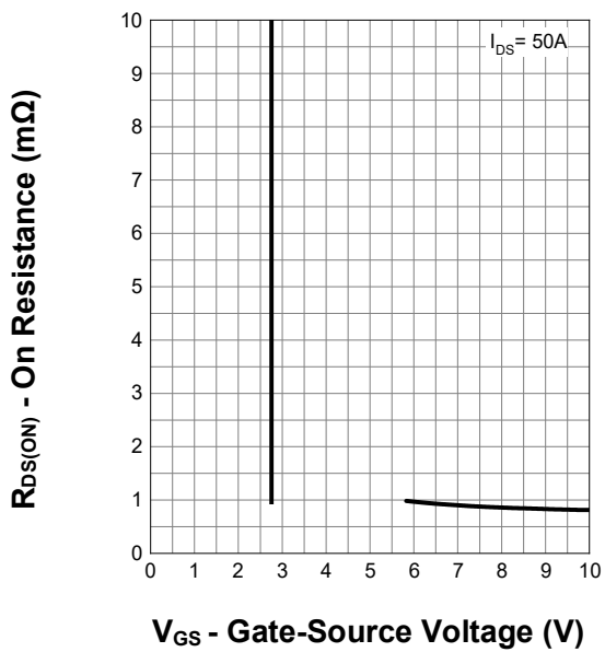
Transfer Characteristics
