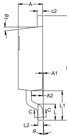
SIDE VIEW(Right)
