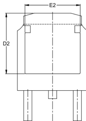
OPTION 1 BOTTOM VIEW
