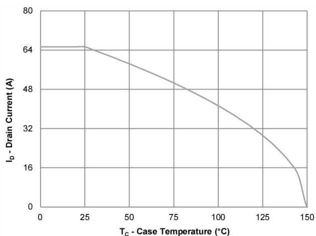
Figure 11: Current Derating
